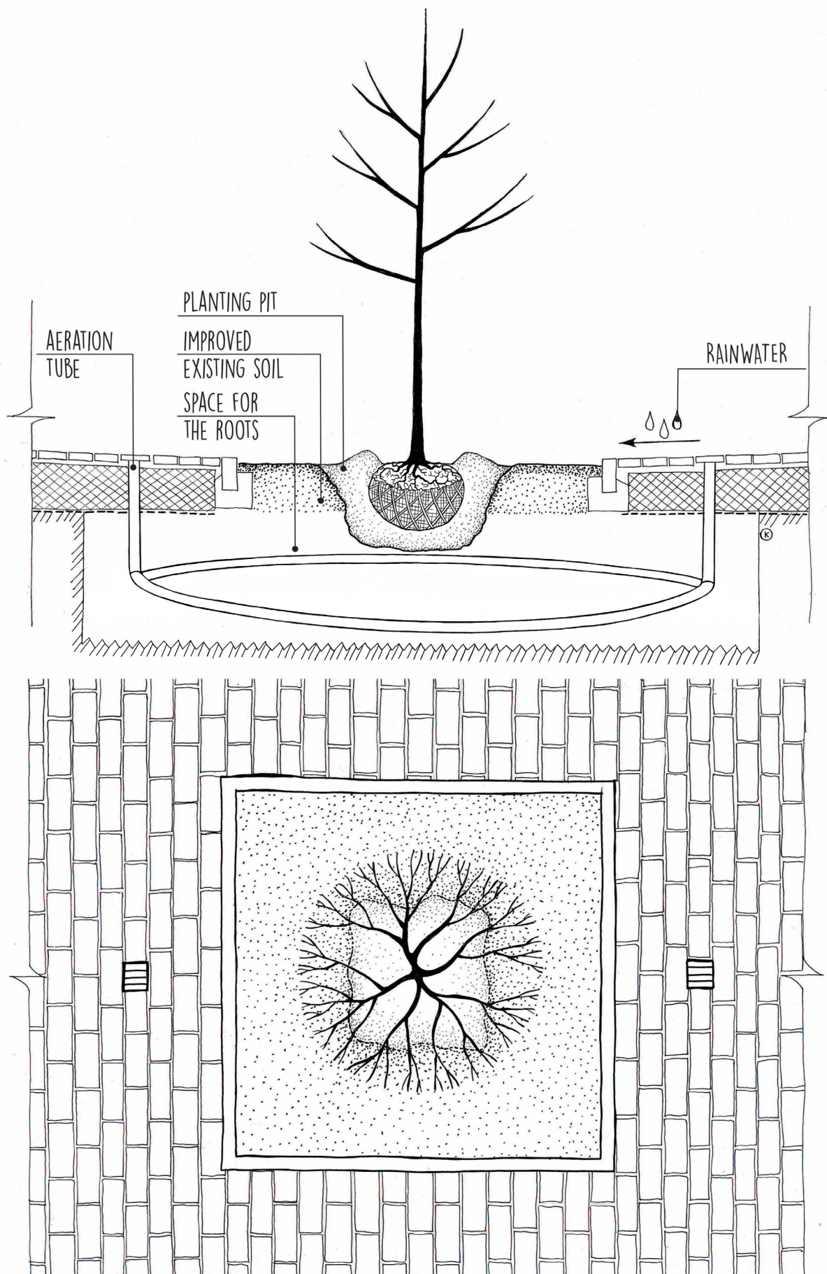
Figure 27: Example of an aeration system.
